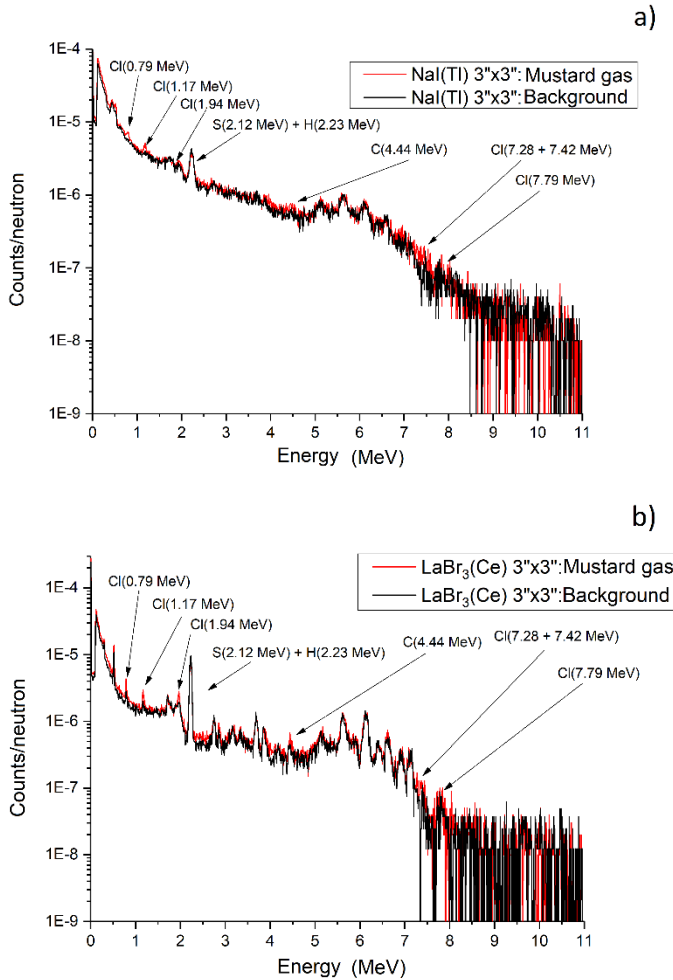
Fig. 4. The energy spectra of the \gamma quanta simulated with the assumption that the detector is made of thallium-activated sodium iodide (a) and cerium-activated lanthanum bromide (b). The red curve shows the simulations using mustard gas, while the black one represents the background noise coming from the surroundings.
