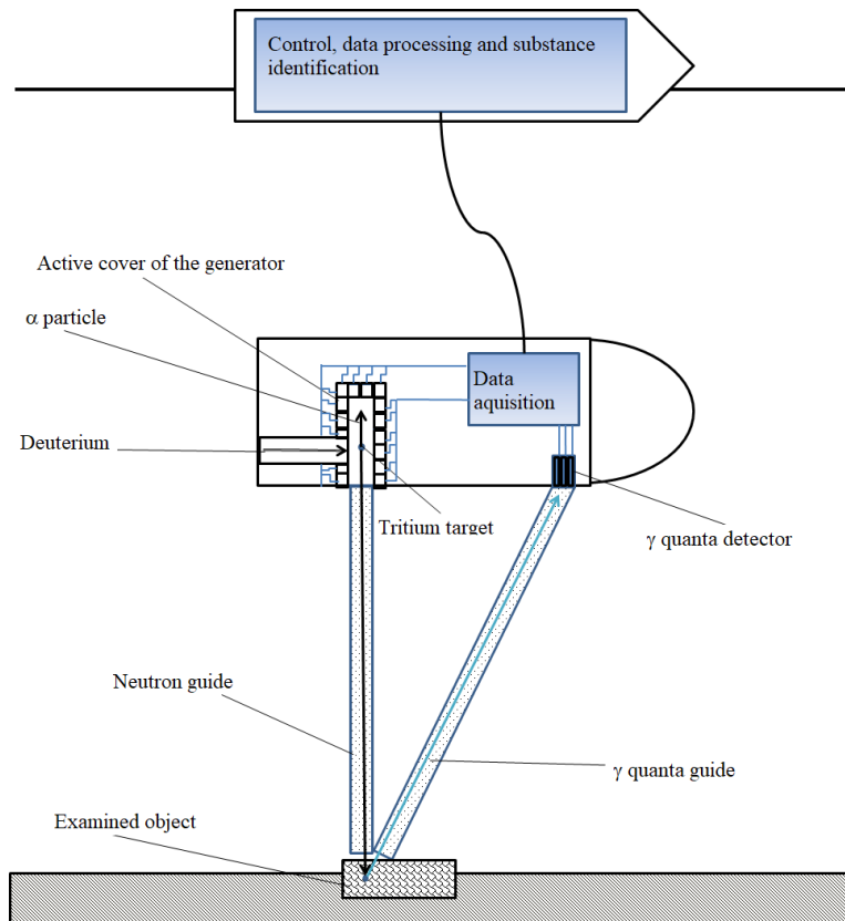
Fig. 2. Diagram of the device being developed within the SABAT project. The underwater drone carrying the compact neutron generator provides a beam that, travelling through the guide, reaches the examined object with no dispersion on the way. Similarly, a fraction of the gamma quanta emitted into the solid angle encompassed by another guide reaches the detector without reacting with the water, facilitating identification. Drawing adapted from [12]
